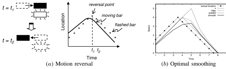
Fig. 2. Motion reversal experiment and optimal smoothing.
