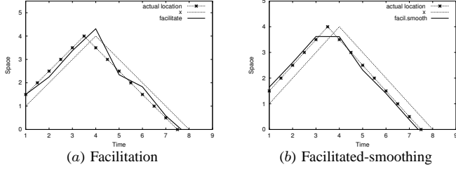
Fig. 4. Perceived trajectory in the facilitation model.
