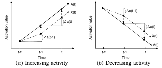
Fig. 3. Facilitatory neural activity.
